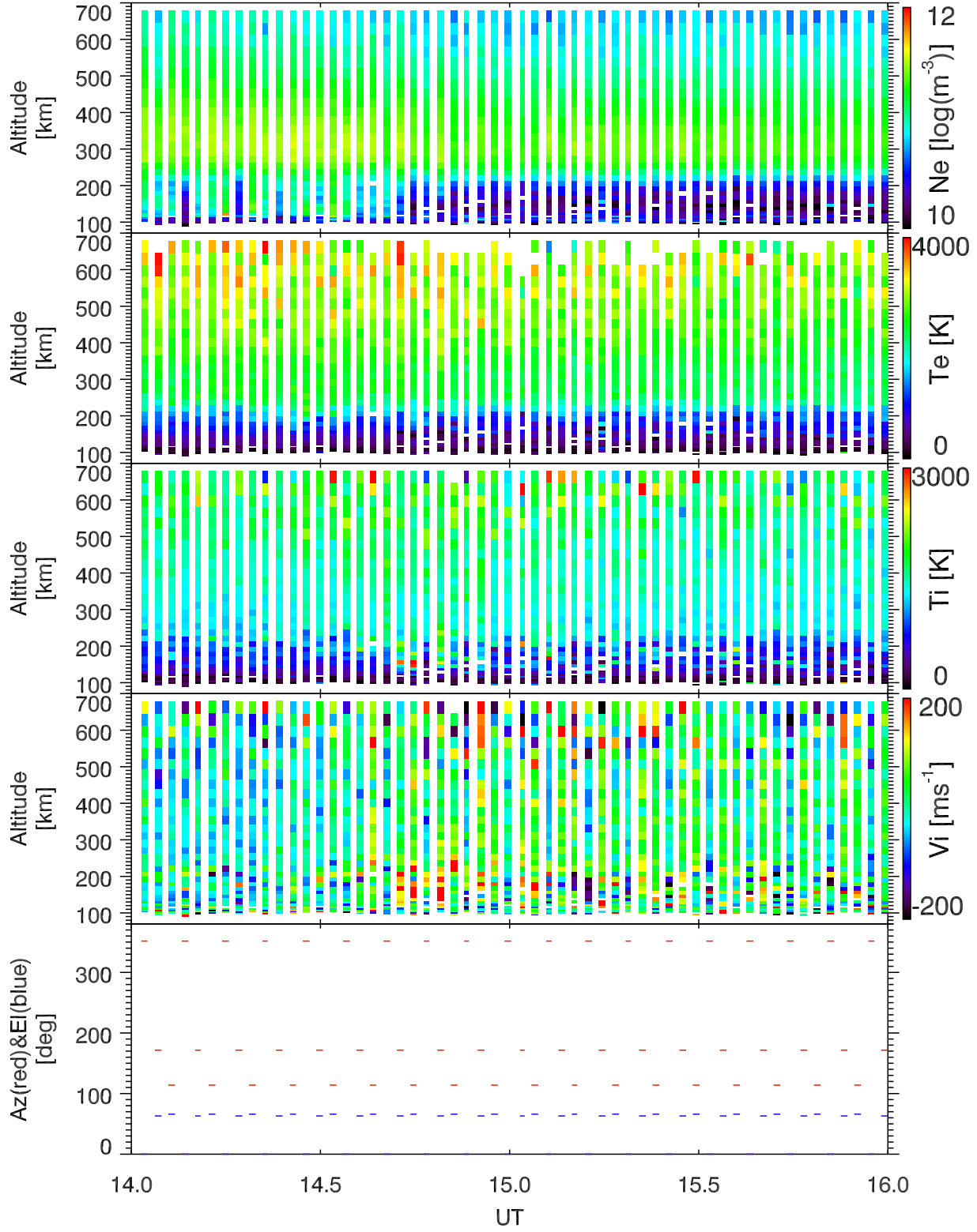
EISCAT 2002-10-09_14_16UT_tau0_ant@32m.
