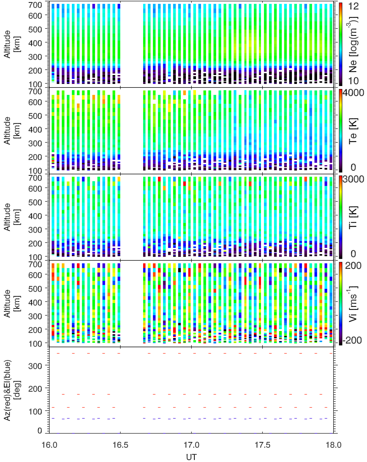
EISCAT 2002-10-09_16_18UT_tau0_ant@32m.
