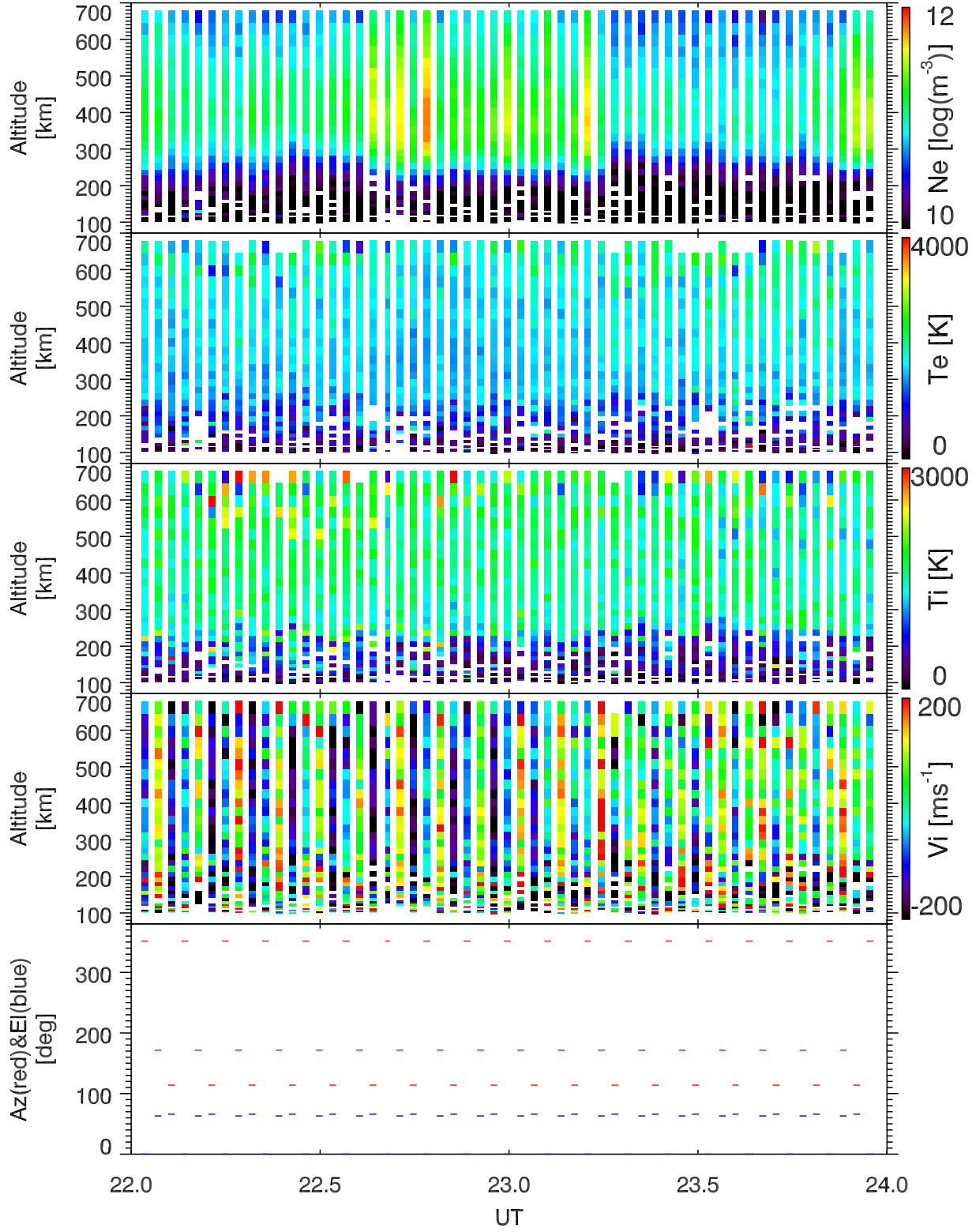
EISCAT 2002-10-09_22_24UT_tau0_ant@32m.
