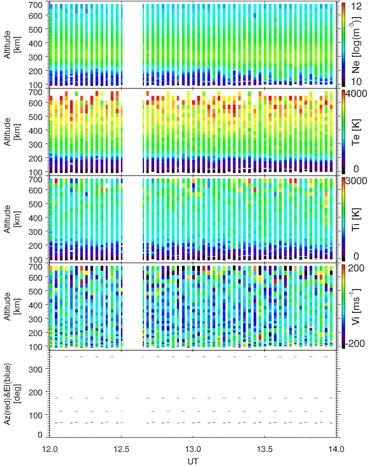
EISCAT 2002-10-10_12_14UT_tau0_ant@32m.
