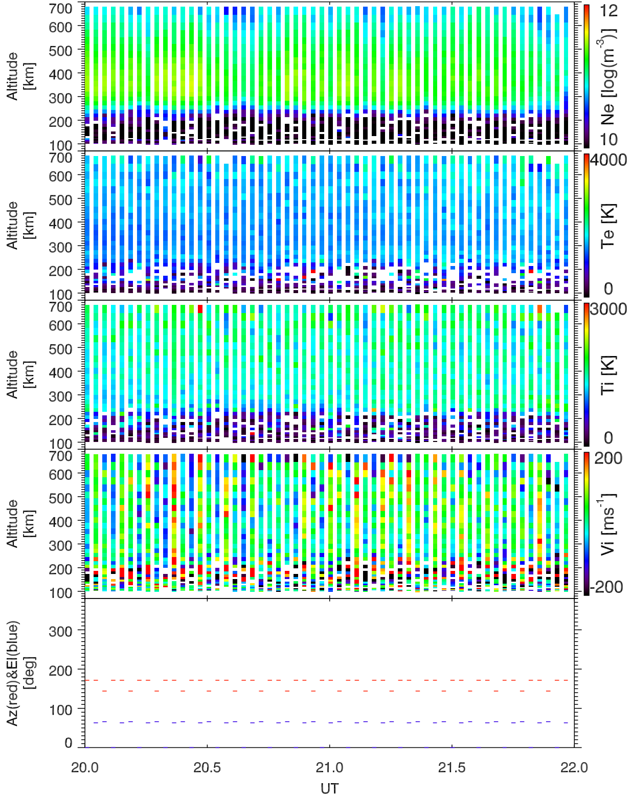
EISCAT 2002-10-10_20_22UT_tau0_ant@32m.
