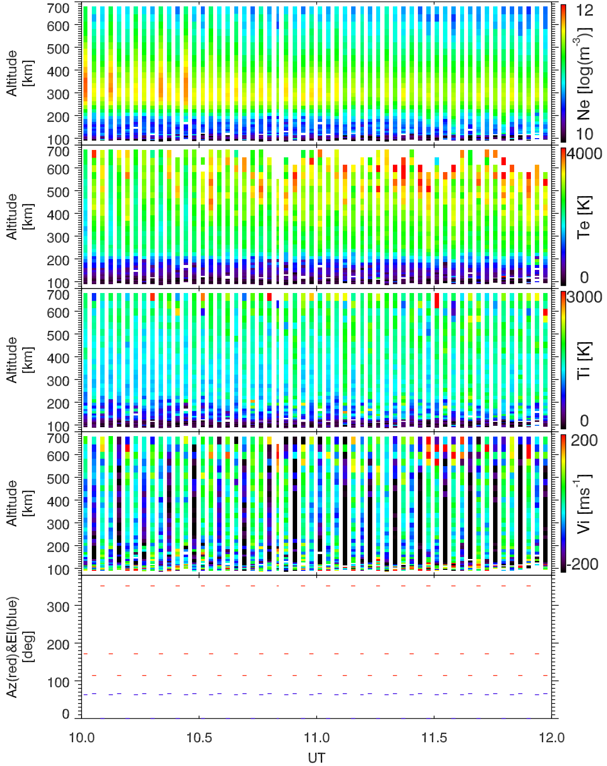
EISCAT 2002-10-13_10_12UT_tau0_ant@32m.
