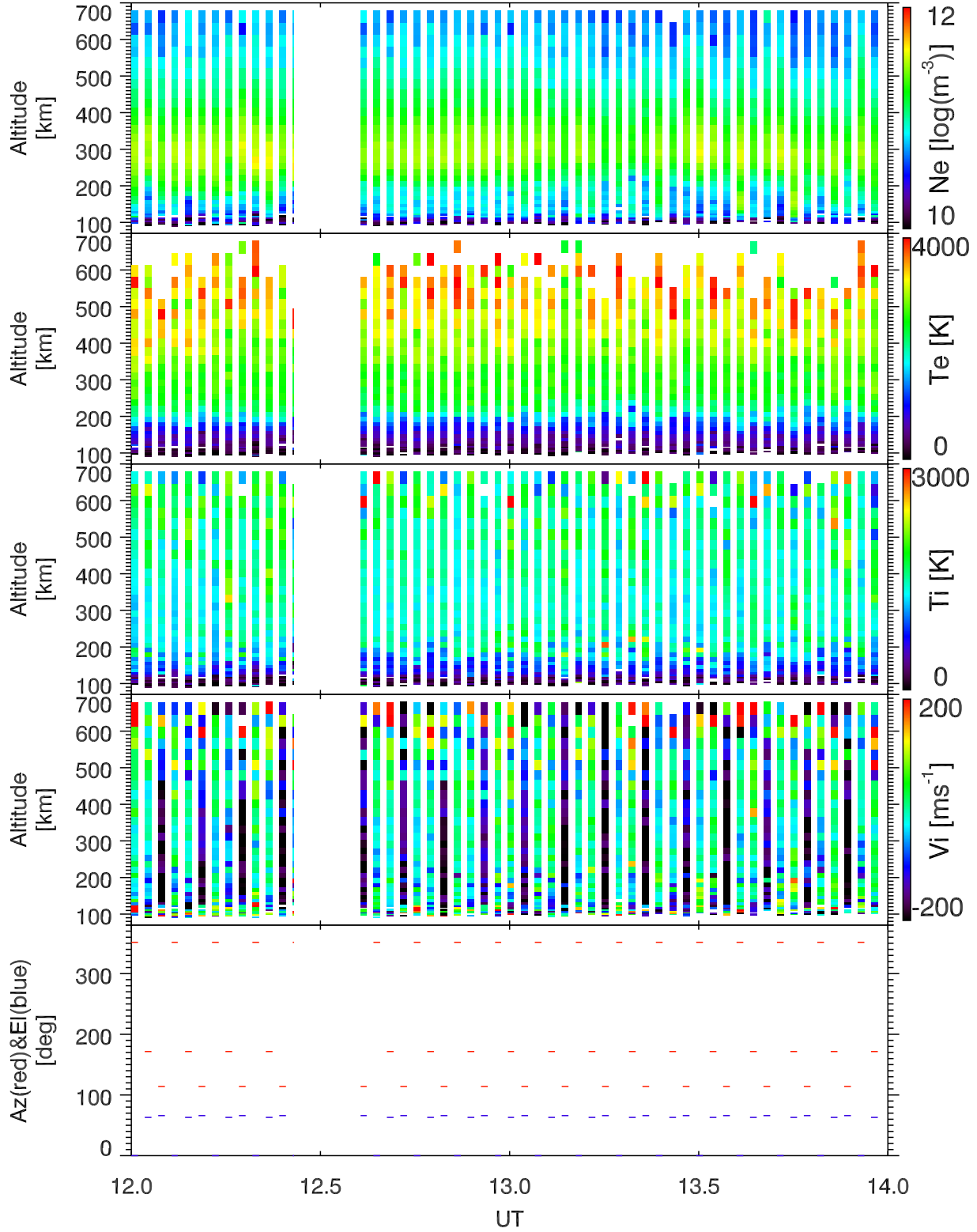
EISCAT 2002-10-13_12_14UT_tau0_ant@32m.
