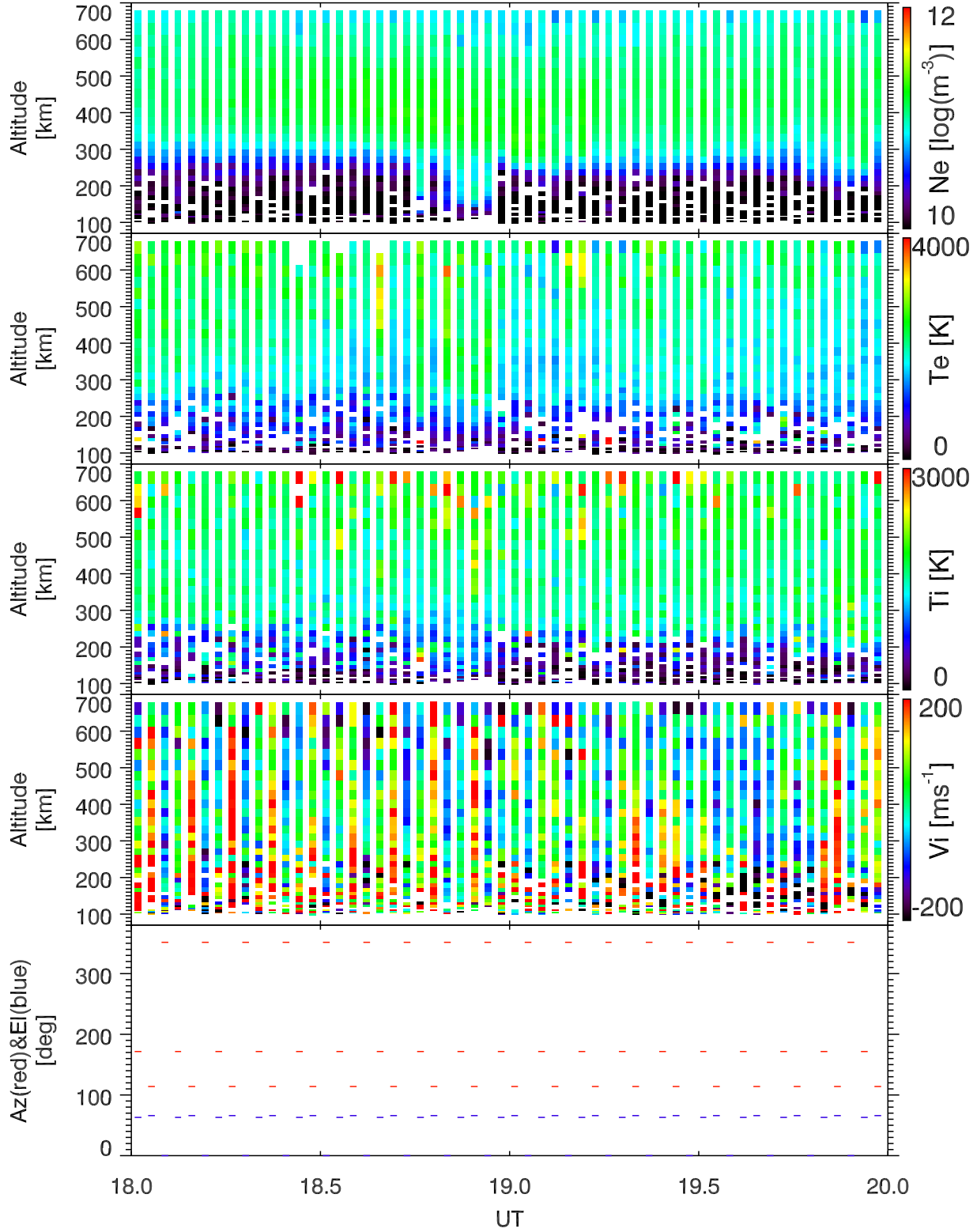
EISCAT 2002-10-14_18_20UT_tau0_ant@32m.
