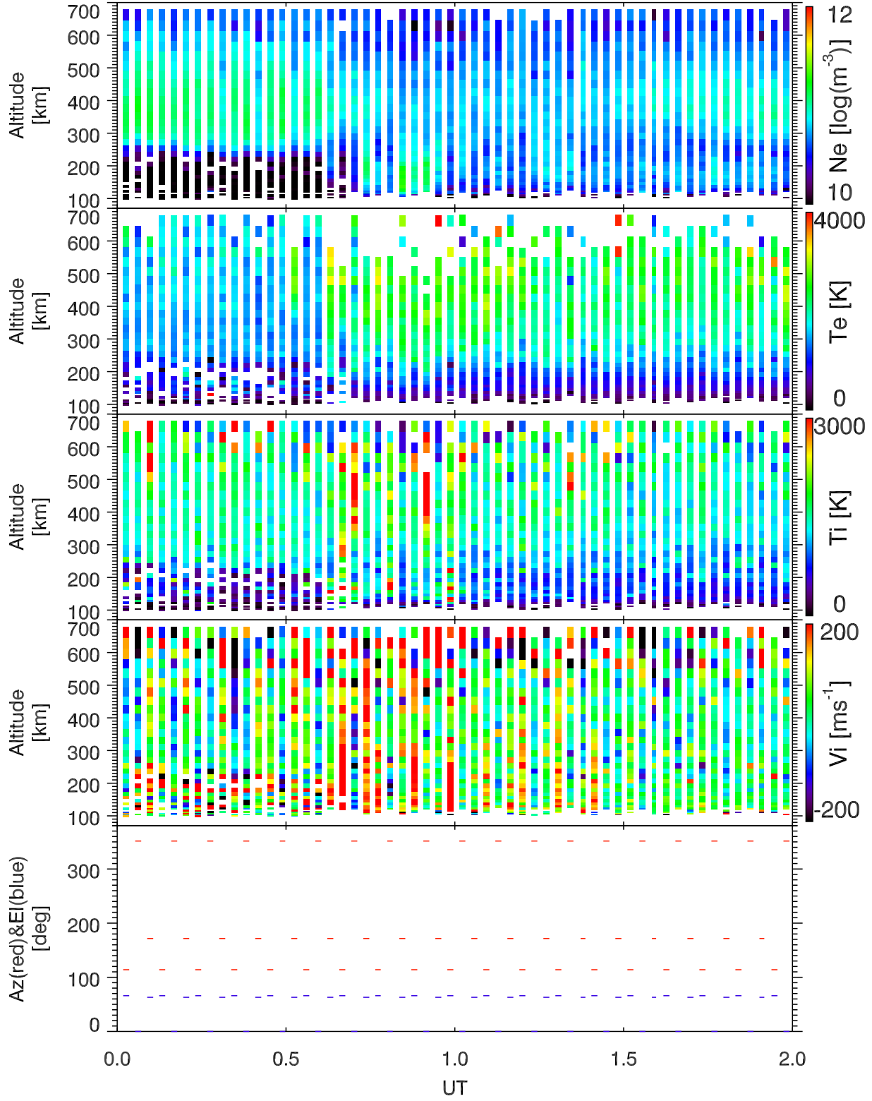
EISCAT 2002-10-15_00_02UT_tau0_ant@32m.
