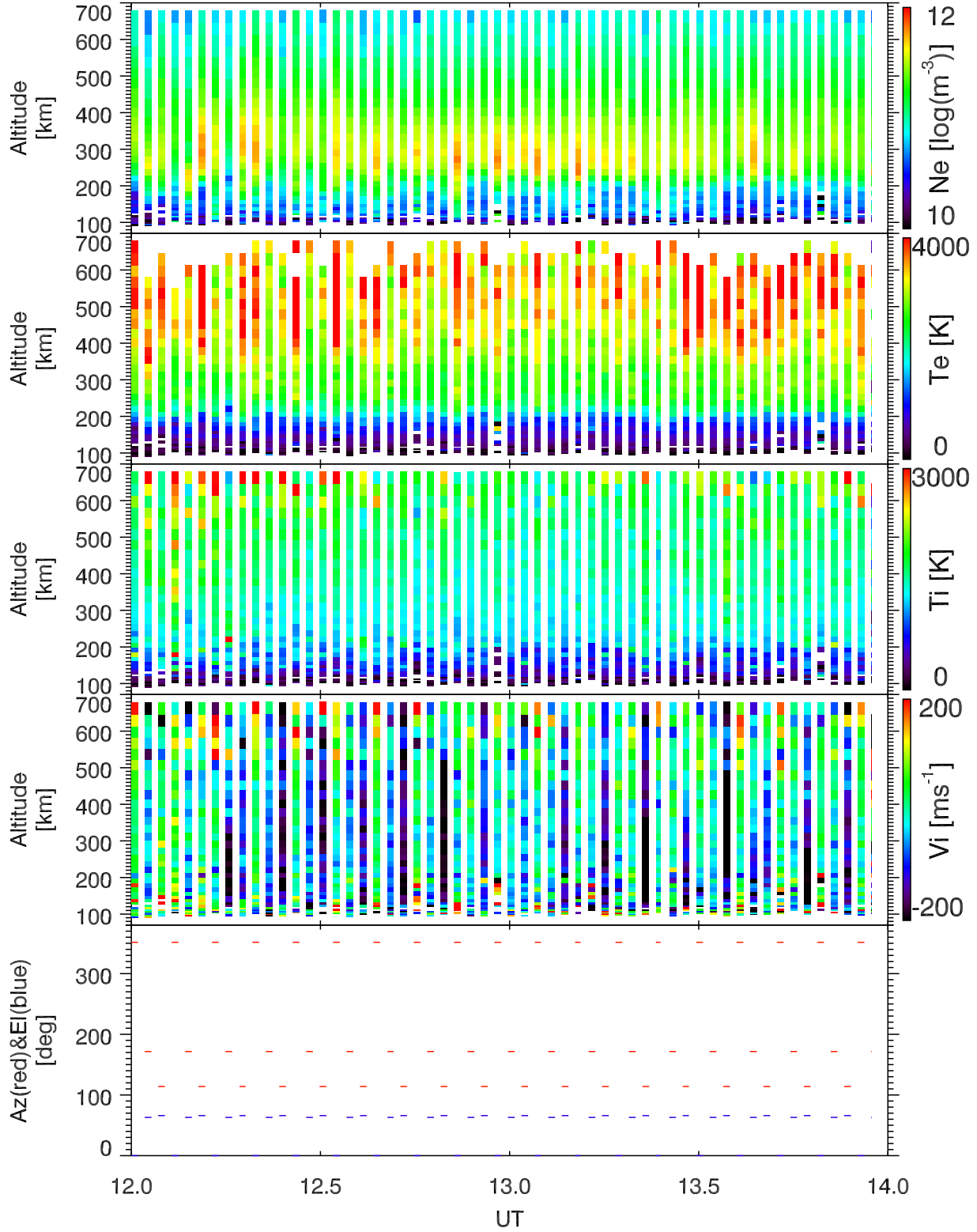
EISCAT 2002-10-15_12_14UT_tau0_ant@32m.
