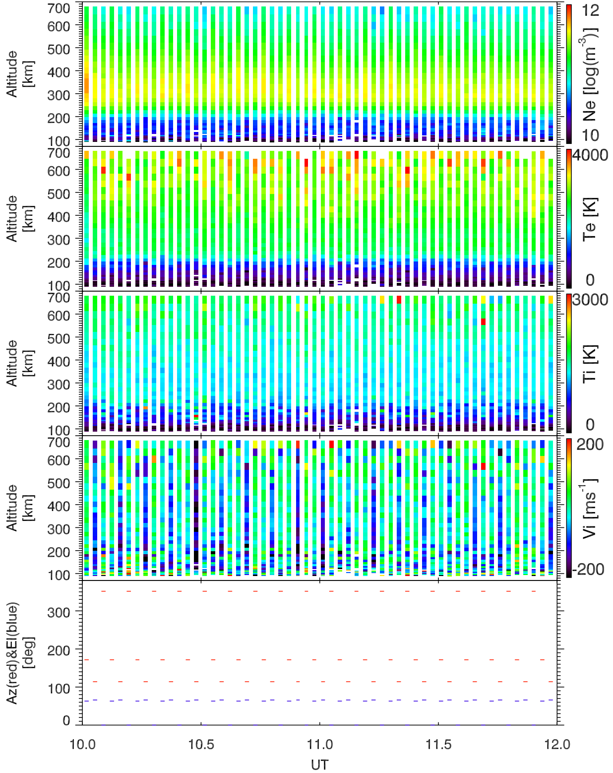
EISCAT 2002-10-17_10_12UT_tau0_ant@32m.
