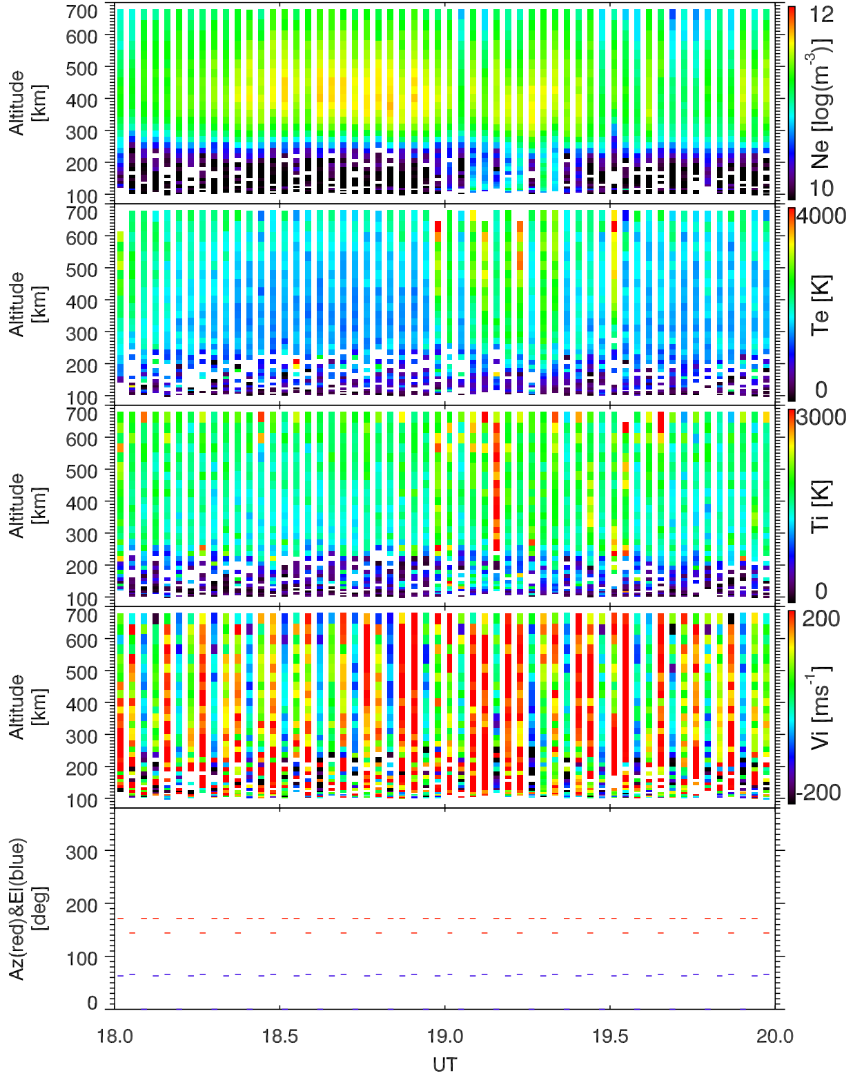
EISCAT 2002-10-18_18_20UT_tau0_ant@32m.
