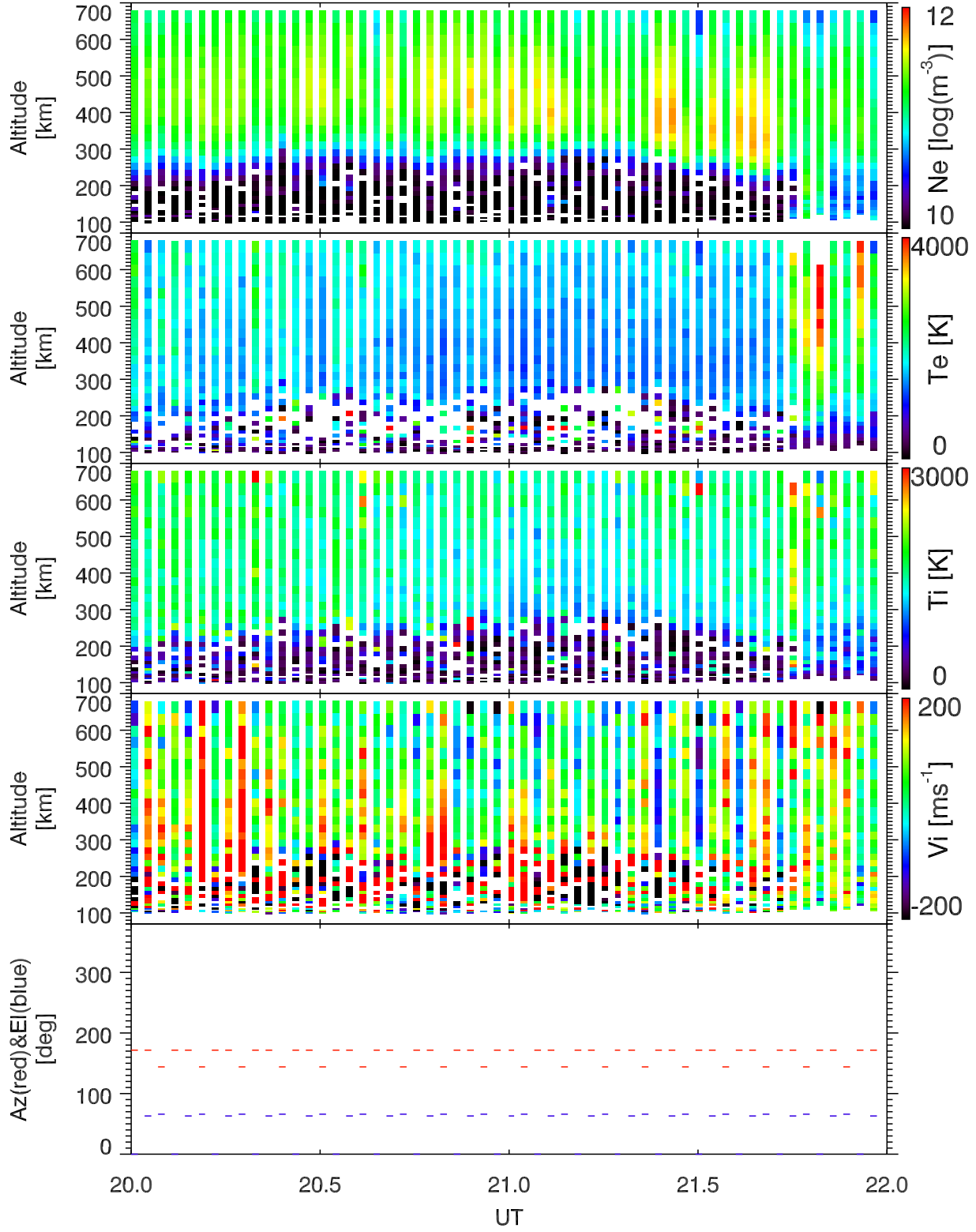
EISCAT 2002-10-18_20_22UT_tau0_ant@32m.
