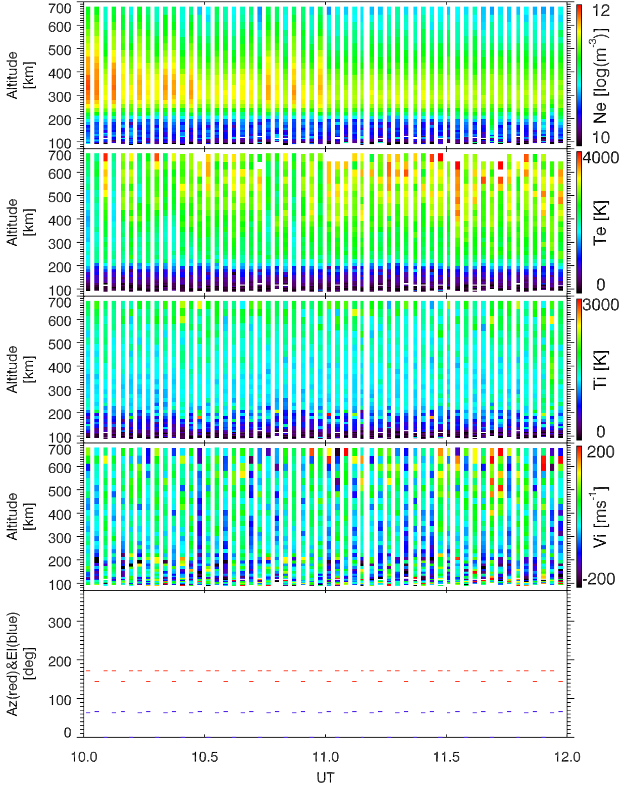
EISCAT 2002-10-19_10_12UT_tau0_ant@32m.
