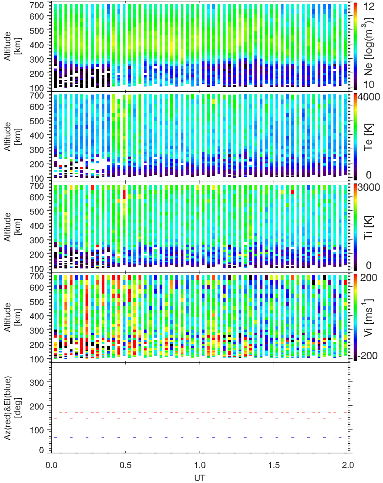
EISCAT 2002-10-20_00_02UT_tau0_ant@32m.
