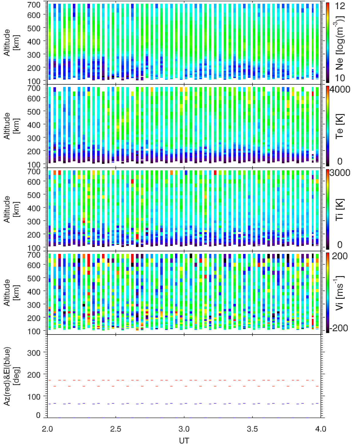
EISCAT 2002-10-20_02_04UT_tau0_ant@32m.
