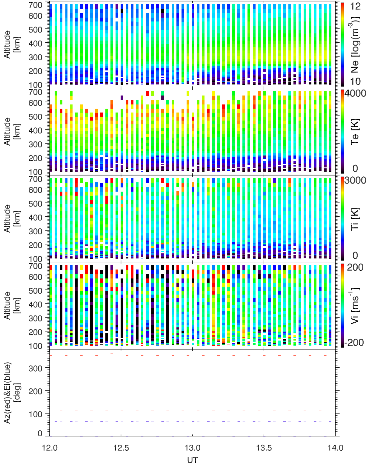
EISCAT 2002-10-20_12_14UT_tau0_ant@32m.
