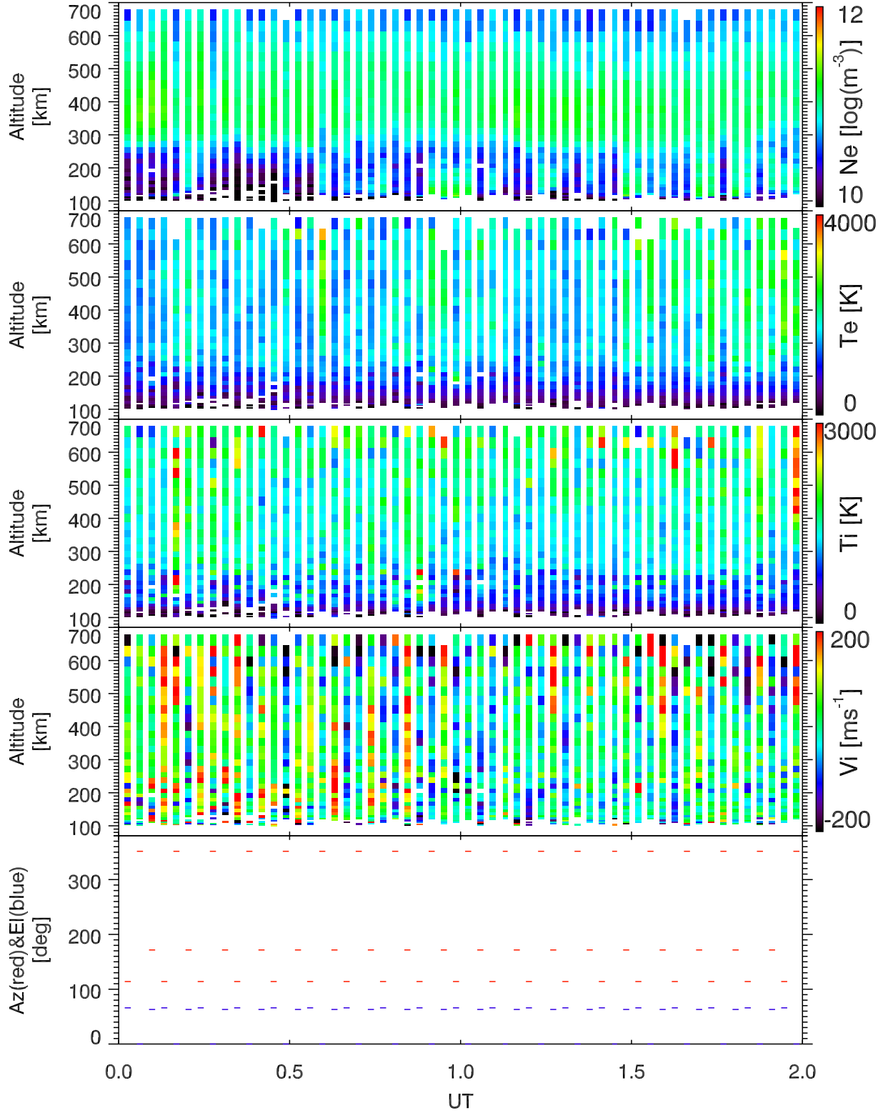
EISCAT 2002-10-21_00_02UT_tau0_ant@32m.
