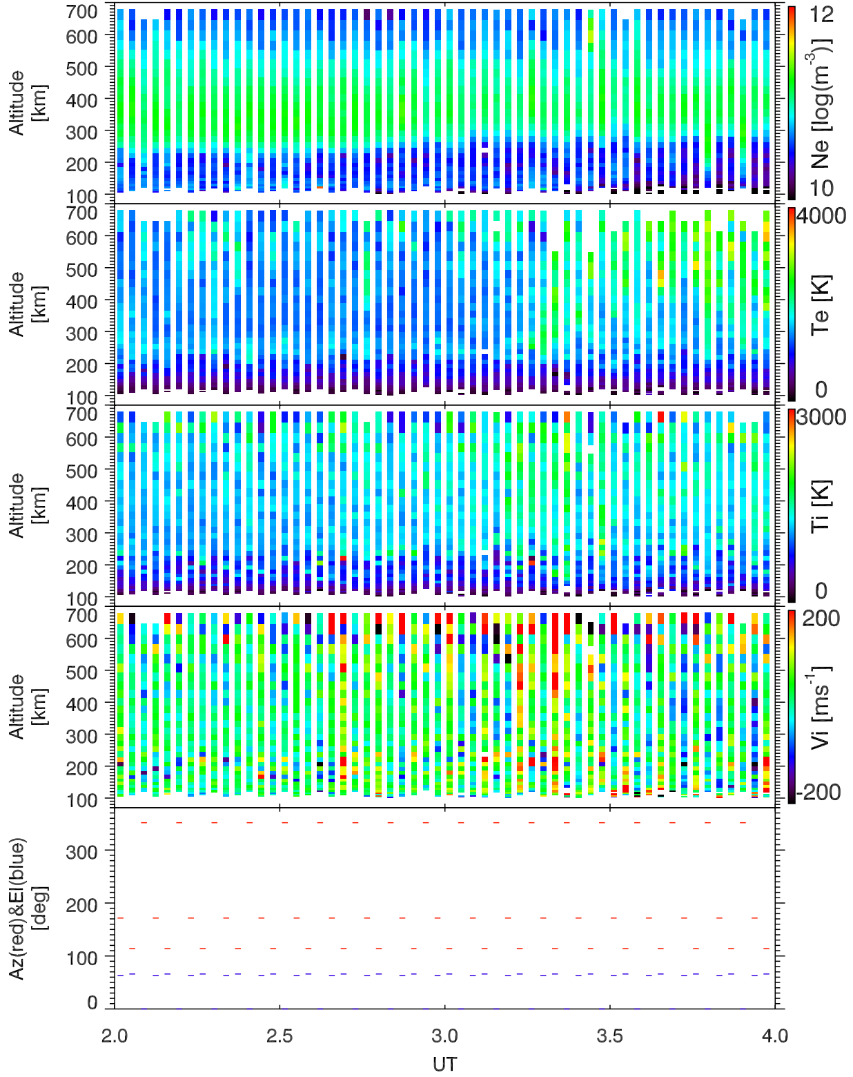
EISCAT 2002-10-22_02_04UT_tau0_ant@32m.
