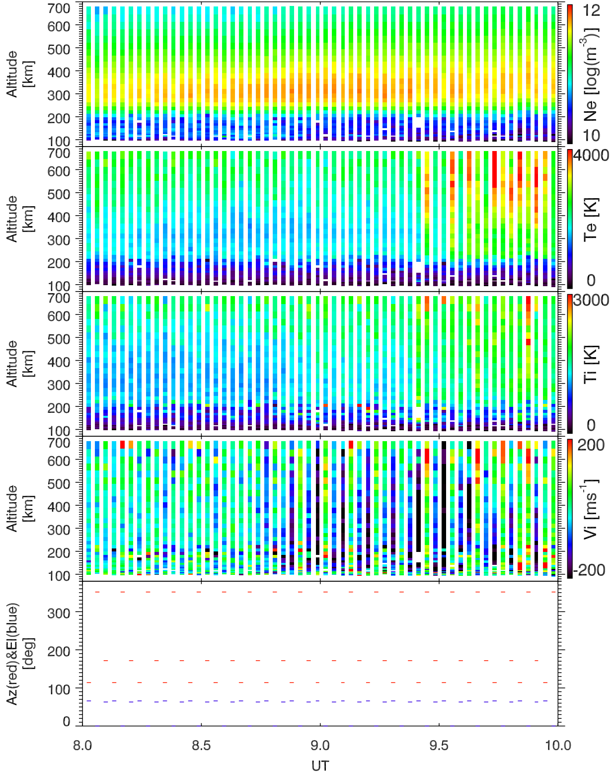
EISCAT 2002-10-22_08_10UT_tau0_ant@32m.
