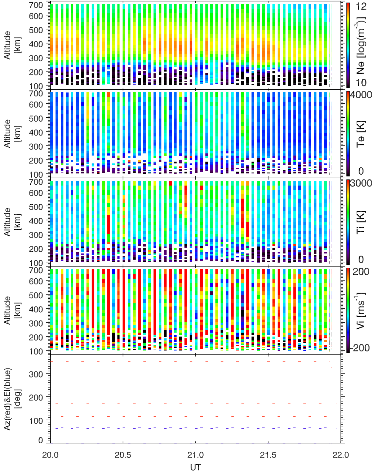
EISCAT 2002-10-22_20_22UT_tau0_ant@32m.
