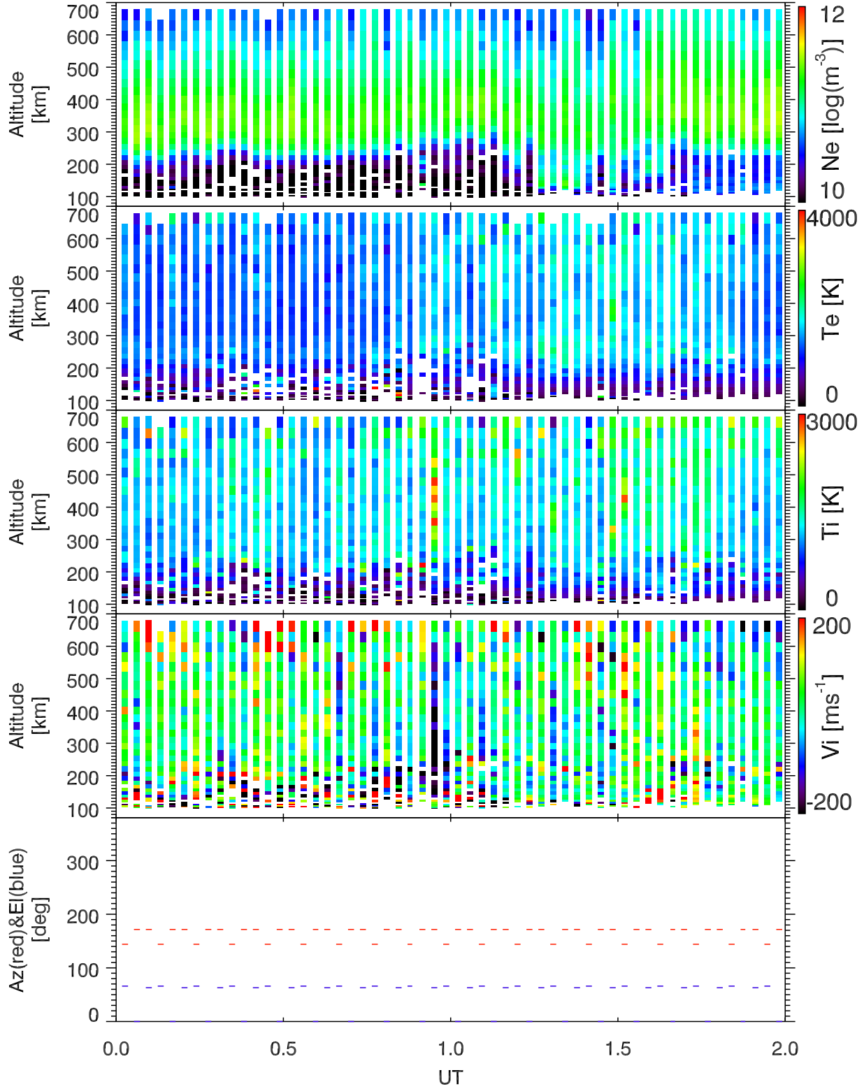
EISCAT 2002-10-23_00_02UT_tau0_ant@32m.
