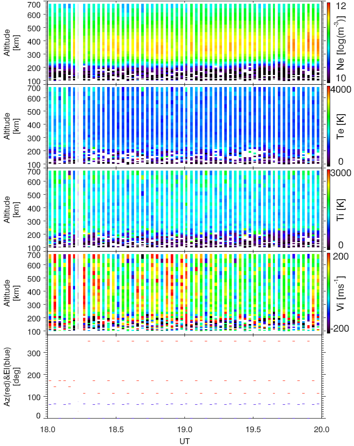
EISCAT 2002-10-23_18_20UT_tau0_ant@32m.
