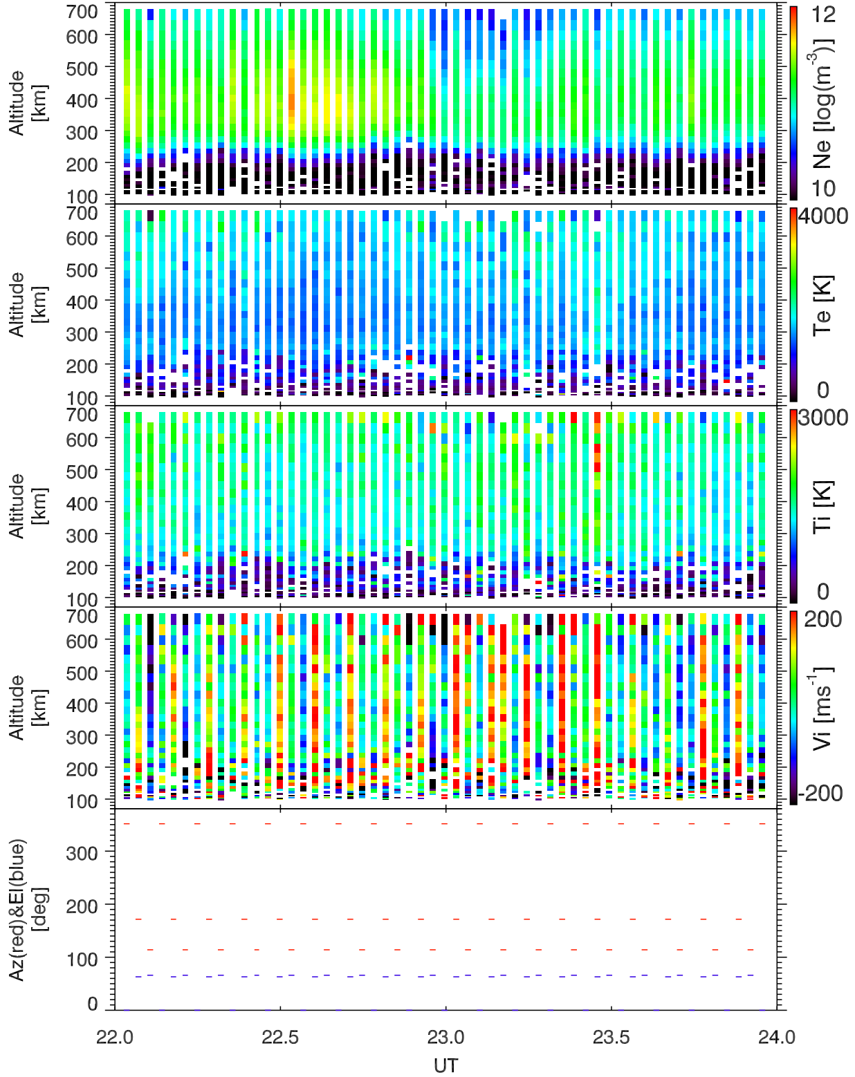
EISCAT 2002-10-23_22_24UT_tau0_ant@32m.
