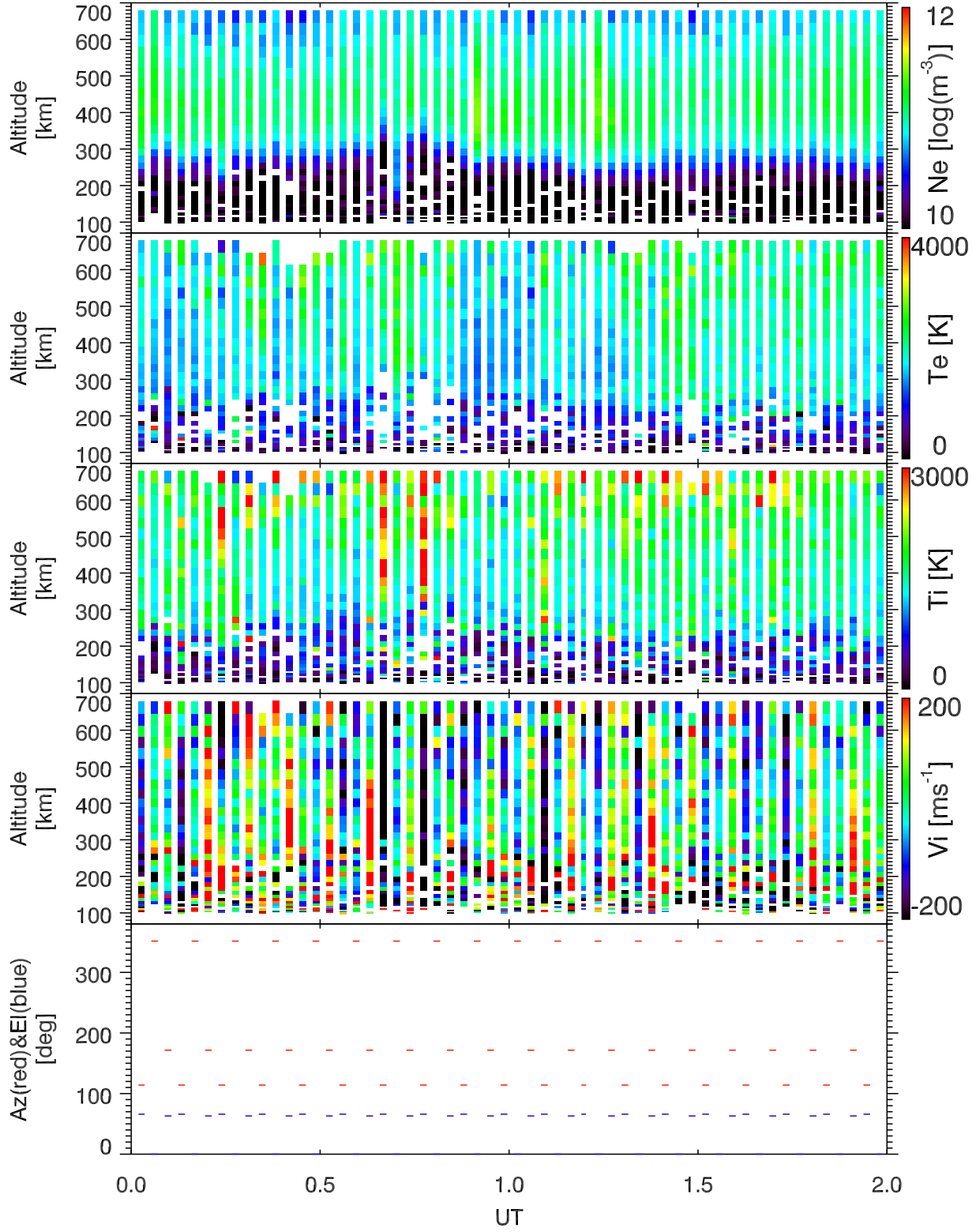
EISCAT 2002-10-24_00_02UT_tau0_ant@32m.
