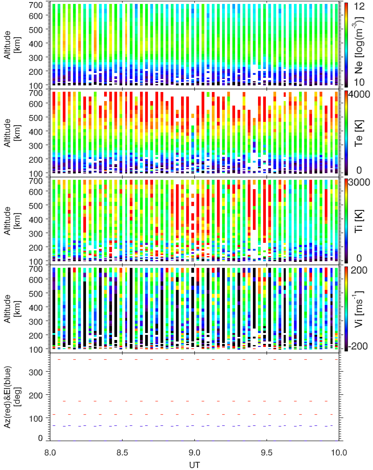
EISCAT 2002-10-24_08_10UT_tau0_ant@32m.
