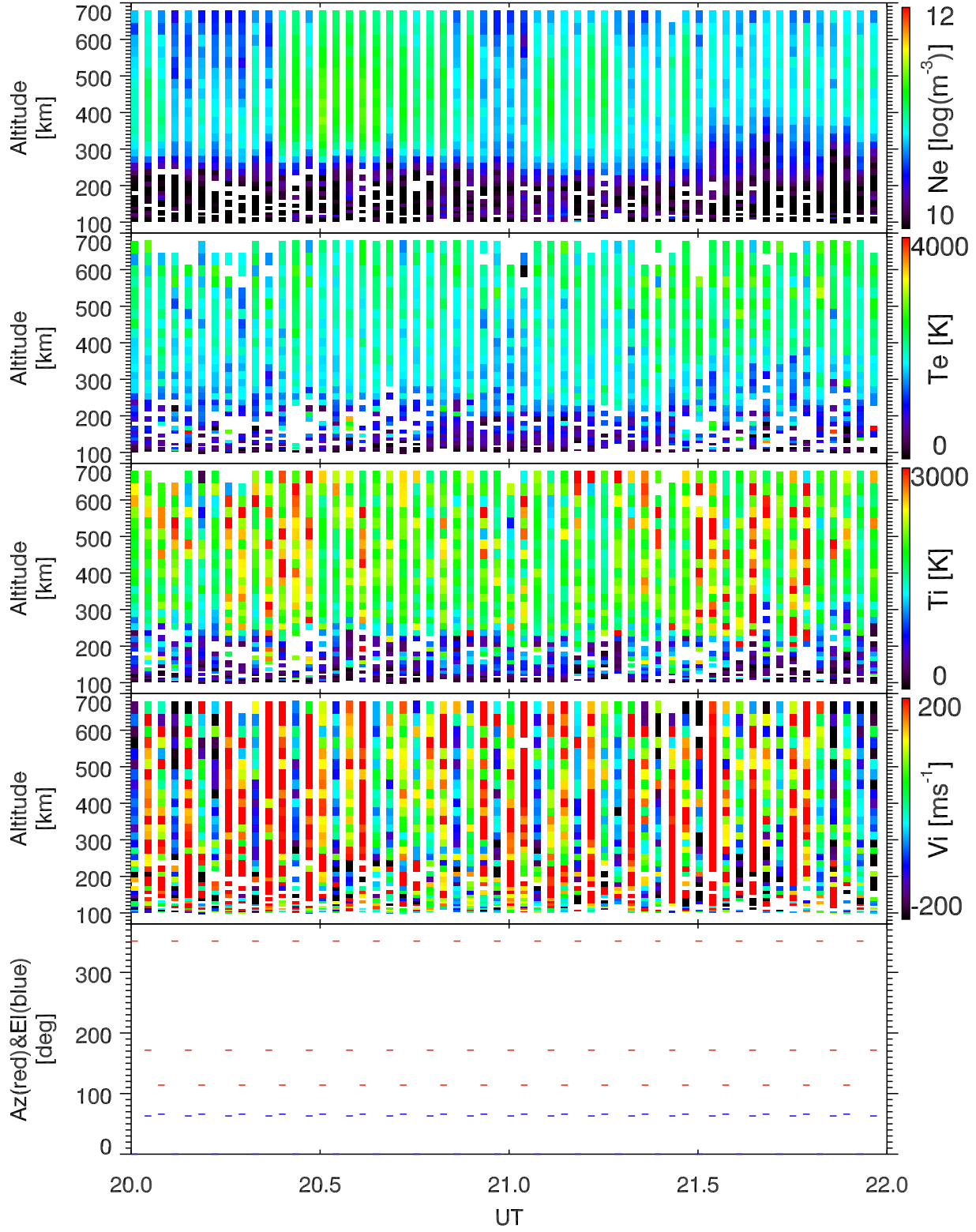
EISCAT 2002-10-24_20_22UT_tau0_ant@32m.
