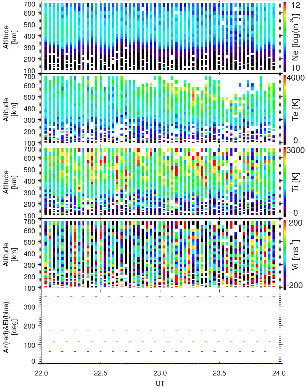
EISCAT 2002-10-24_22_24UT_tau0_ant@32m.
