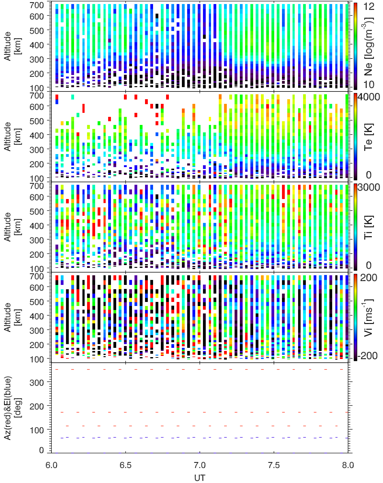
EISCAT 2002-10-25_06_08UT_tau0_ant@32m.
