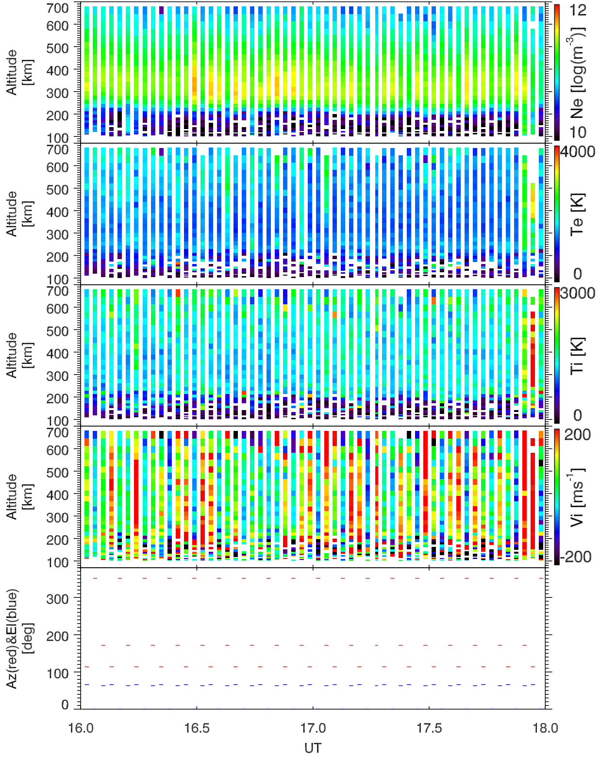
EISCAT 2002-10-26_16_18UT_tau0_ant@32m.
