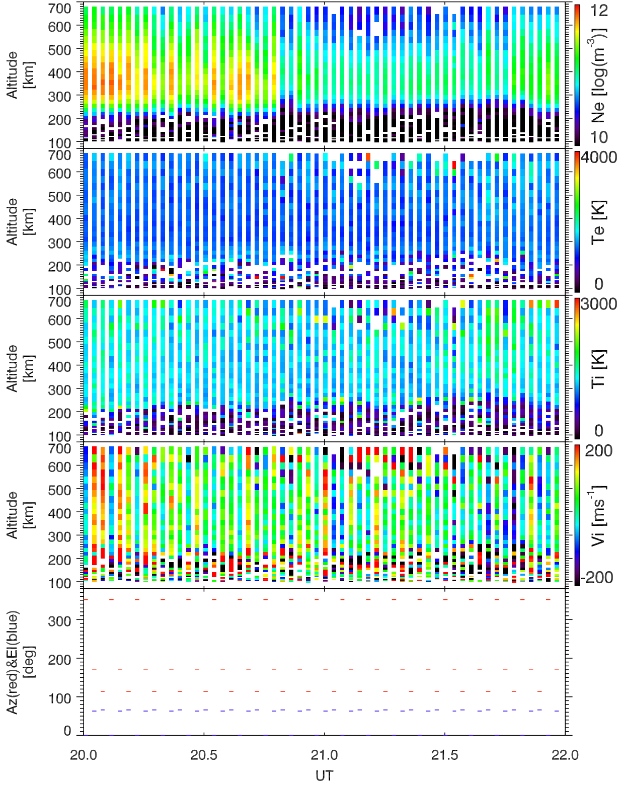
EISCAT 2002-10-26_20_22UT_tau0_ant@32m.
