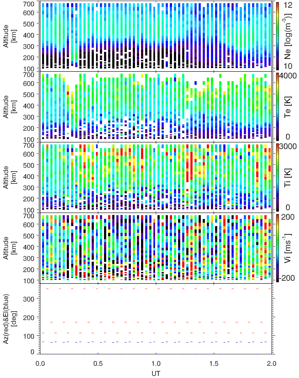
EISCAT 2002-10-27_00_02UT_tau0_ant@32m.
