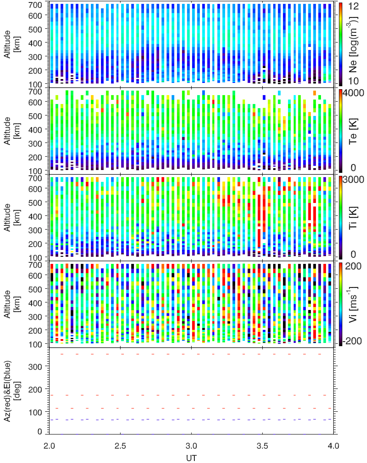
EISCAT 2002-10-27_02_04UT_tau0_ant@32m.
