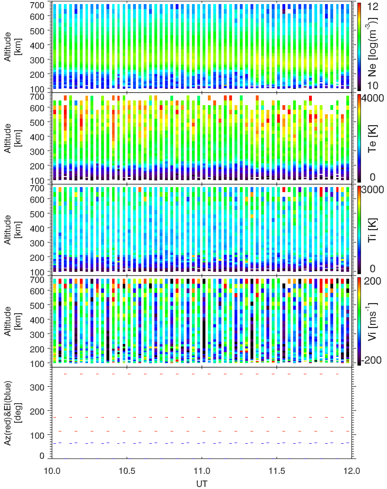
EISCAT 2002-10-27_10_12UT_tau0_ant@32m.
