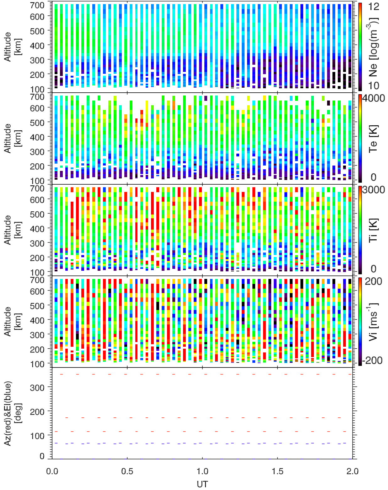
EISCAT 2002-10-28_00_02UT_tau0_ant@32m.
