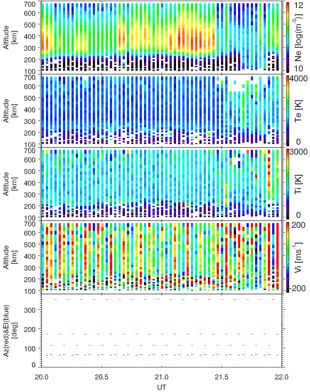
EISCAT 2002-10-28_20_22UT_tau0_ant@32m.
