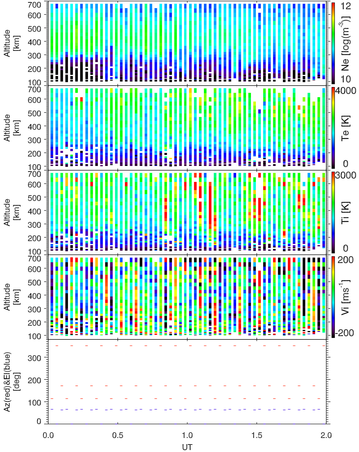
EISCAT 2002-10-29_00_02UT_tau0_ant@32m.
