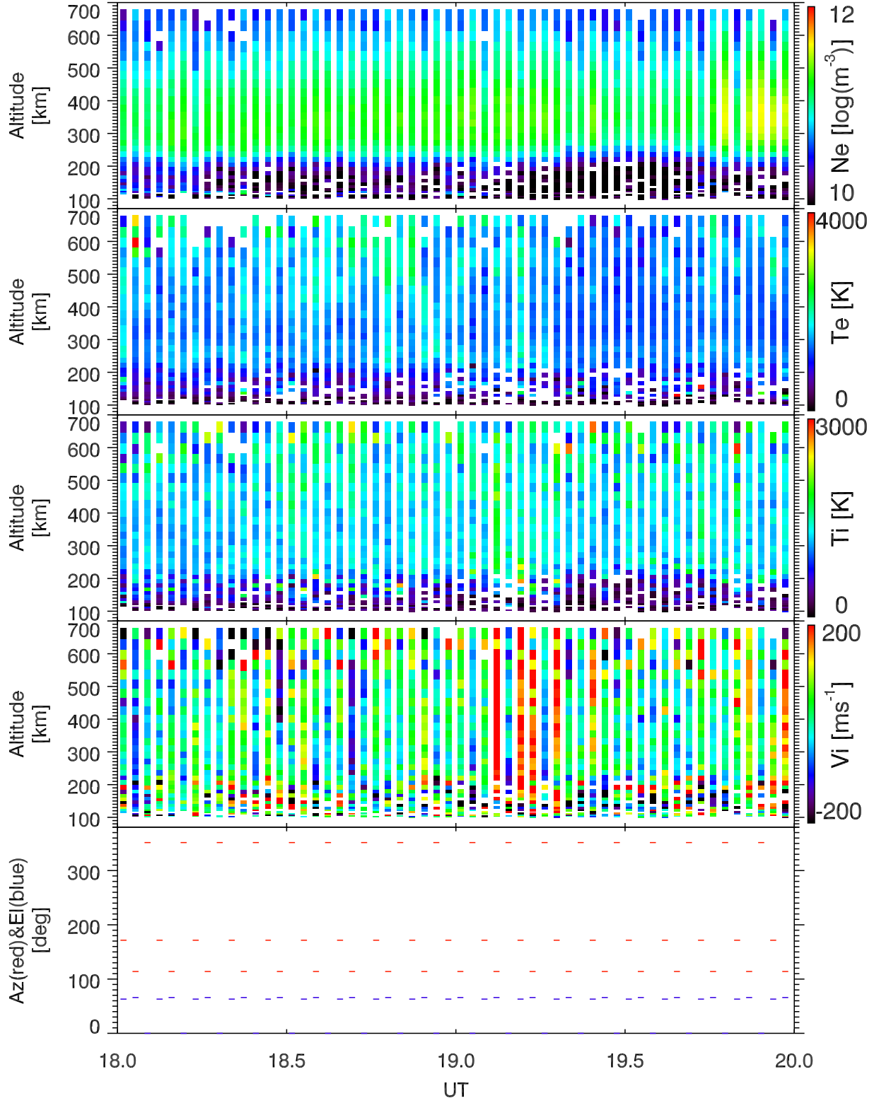
EISCAT 2002-10-29_18_20UT_tau0_ant@32m.
