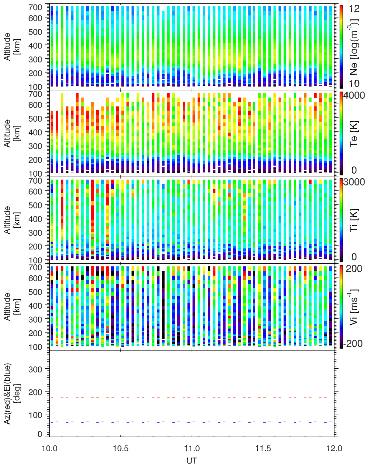
EISCAT 2002-10-30_10_12UT_tau0_ant@32m.
