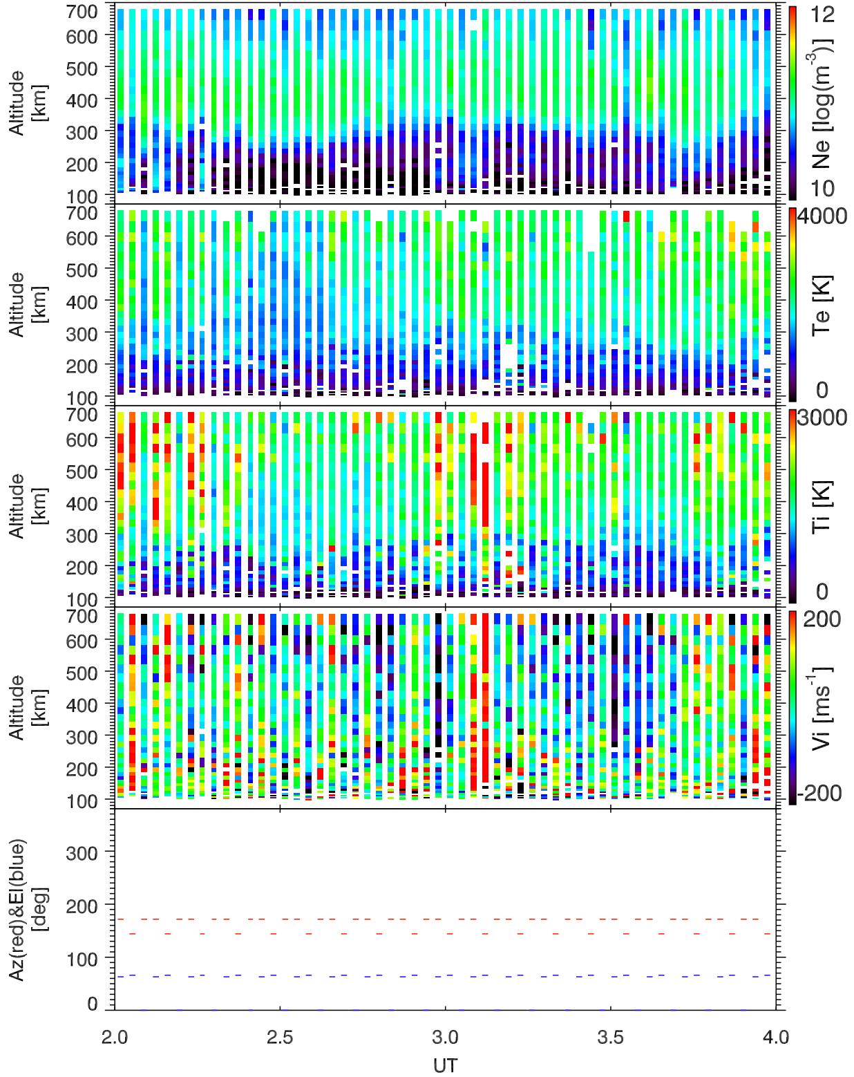
EISCAT 2002-10-31_02_04UT_tau0_ant@32m.
