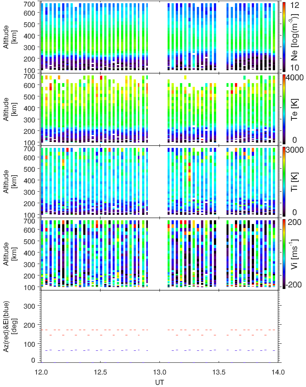
EISCAT 2002-10-31_12_14UT_tau0_ant@32m.
