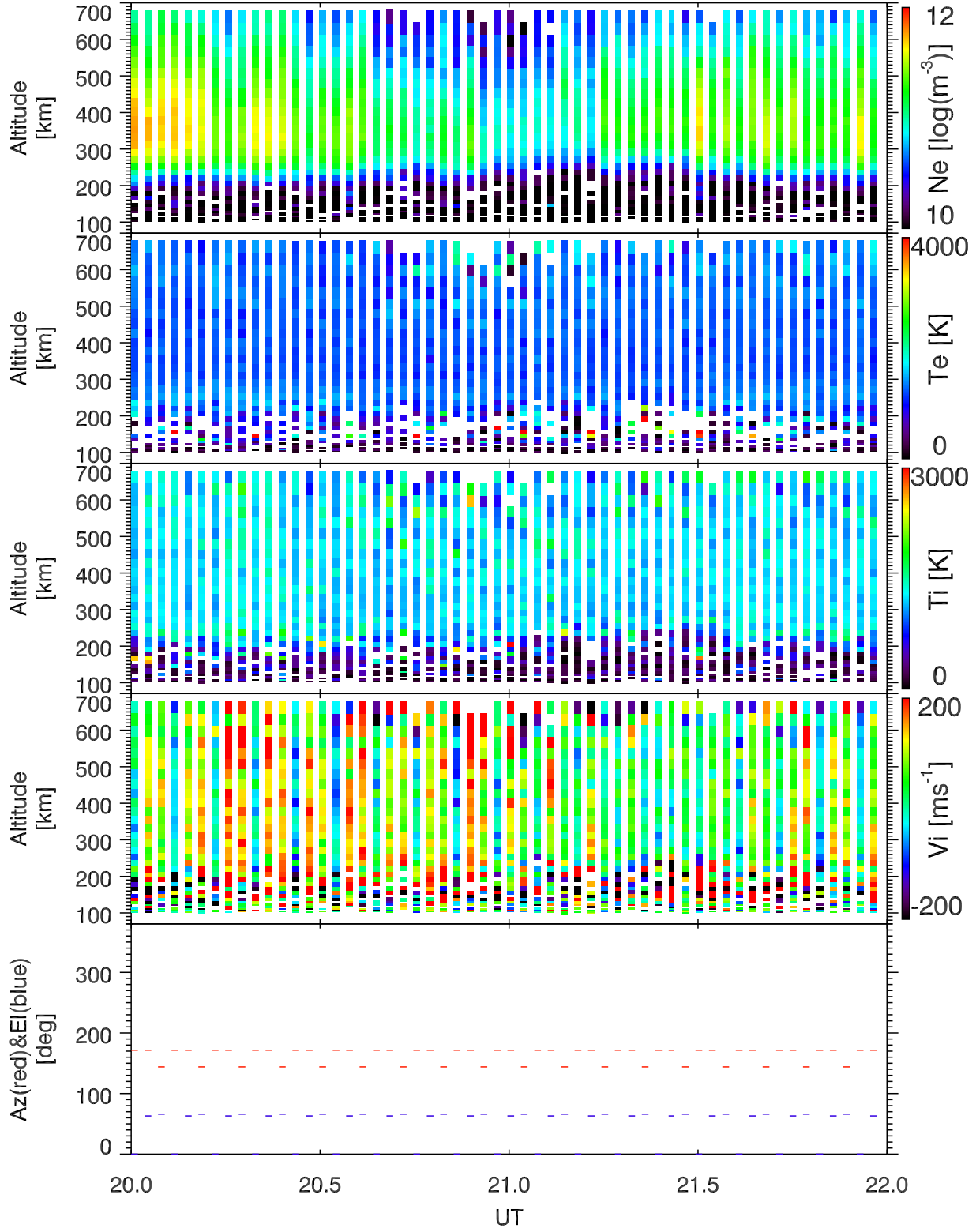
EISCAT 2002-10-31_20_22UT_tau0_ant@32m.
