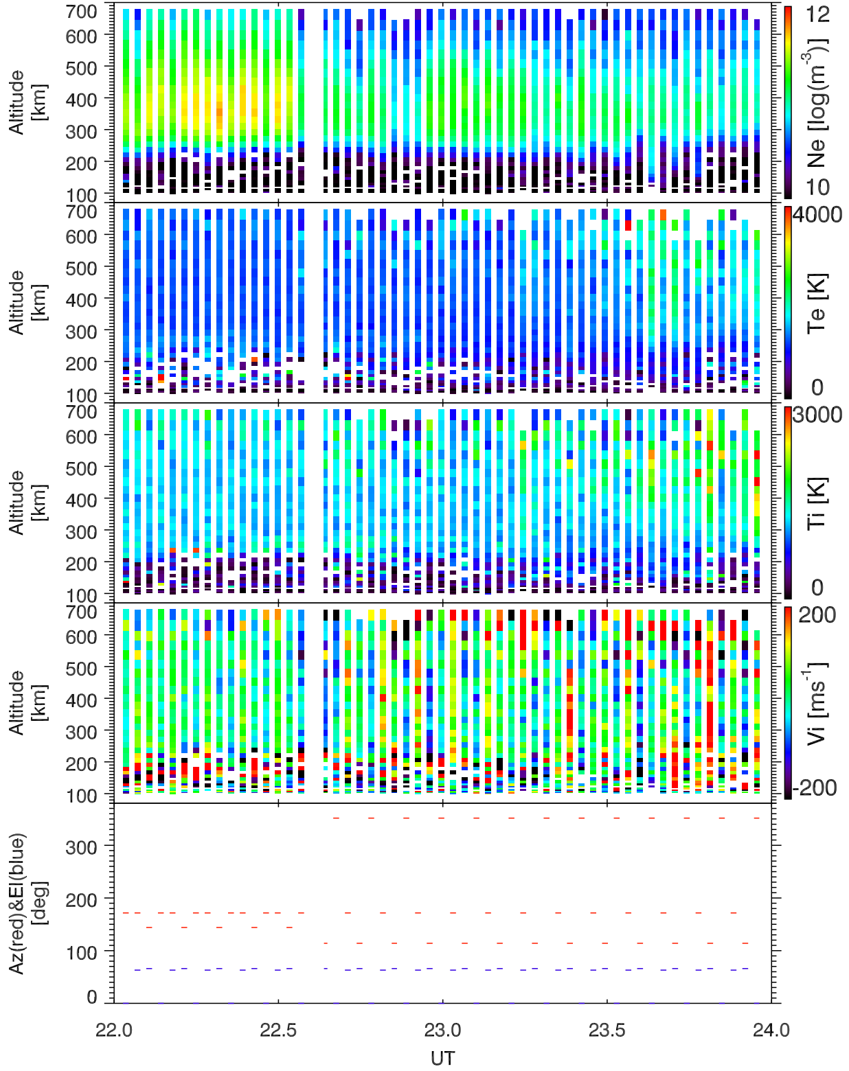
EISCAT 2002-10-31_22_24UT_tau0_ant@32m.
