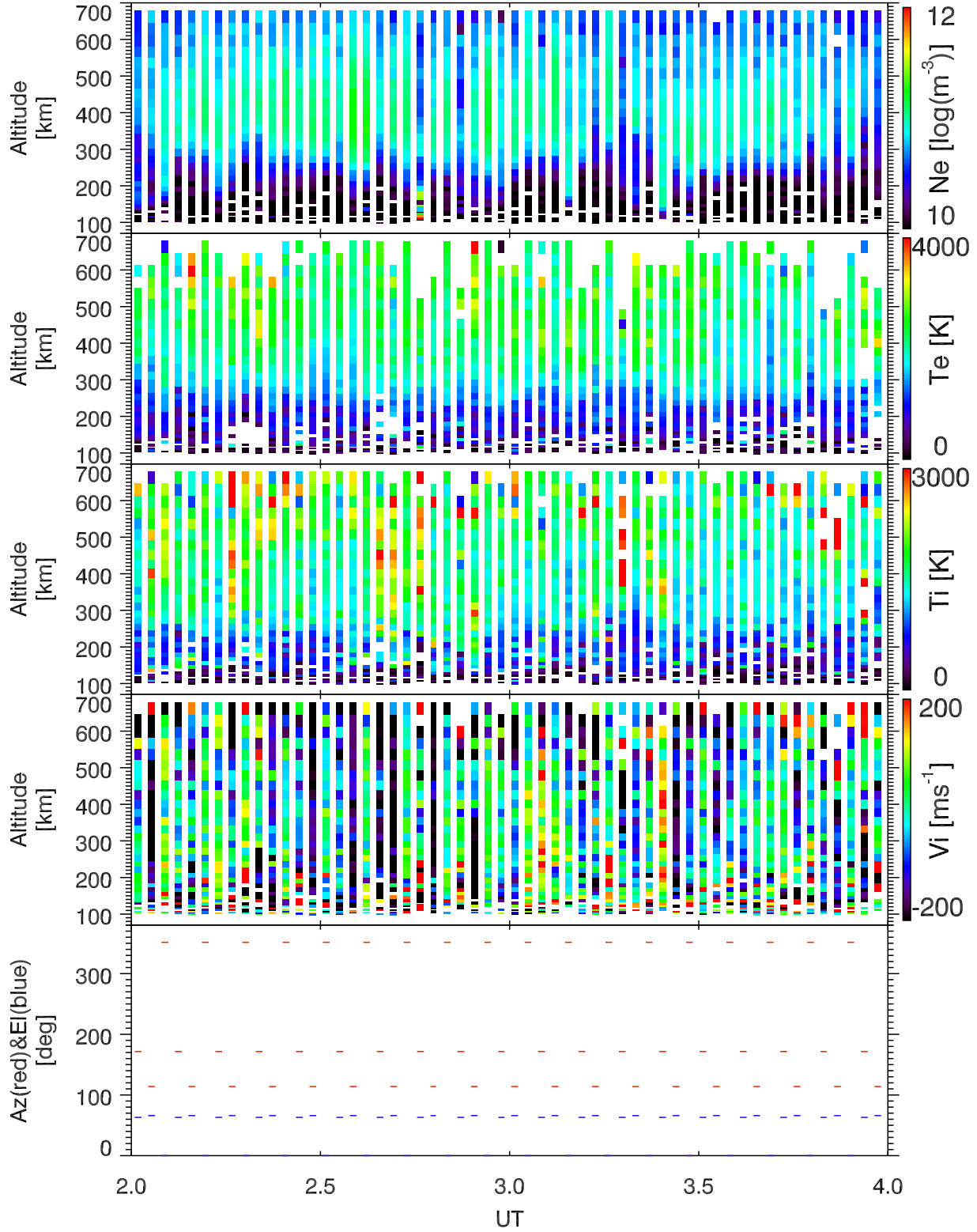
EISCAT 2002-11-01_02_04UT_tau0_ant@32m.
