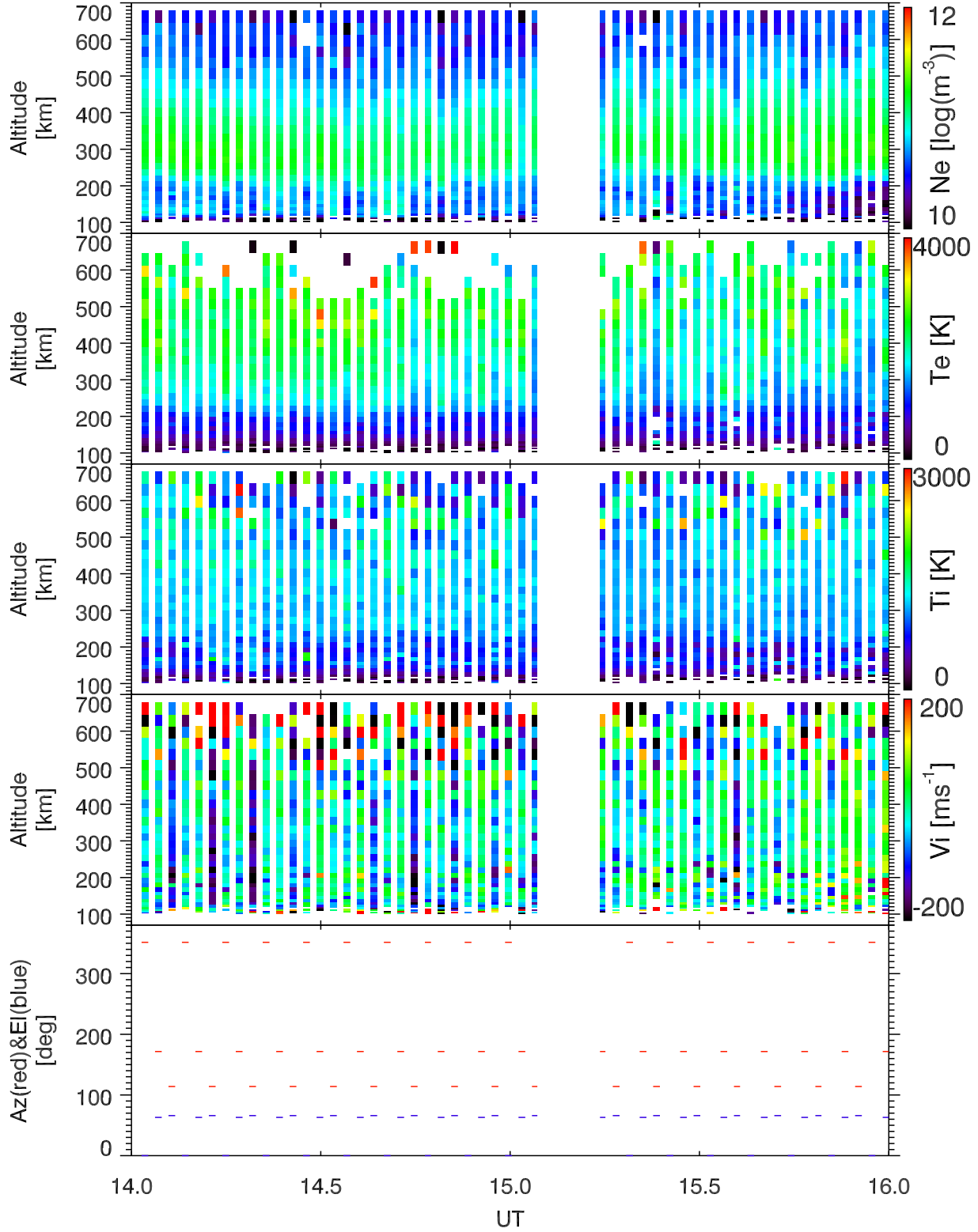
EISCAT 2002-11-01_14_16UT_tau0_ant@32m.
