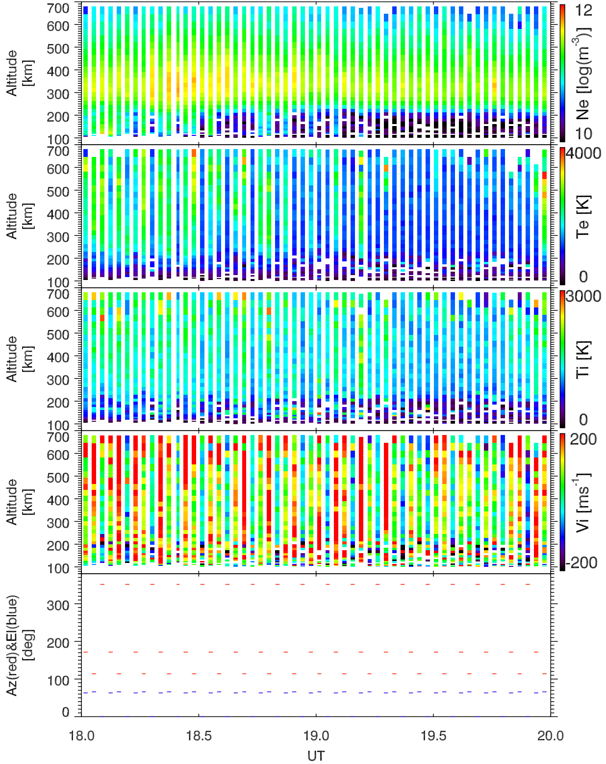
EISCAT 2002-11-01_18_20UT_tau0_ant@32m.
