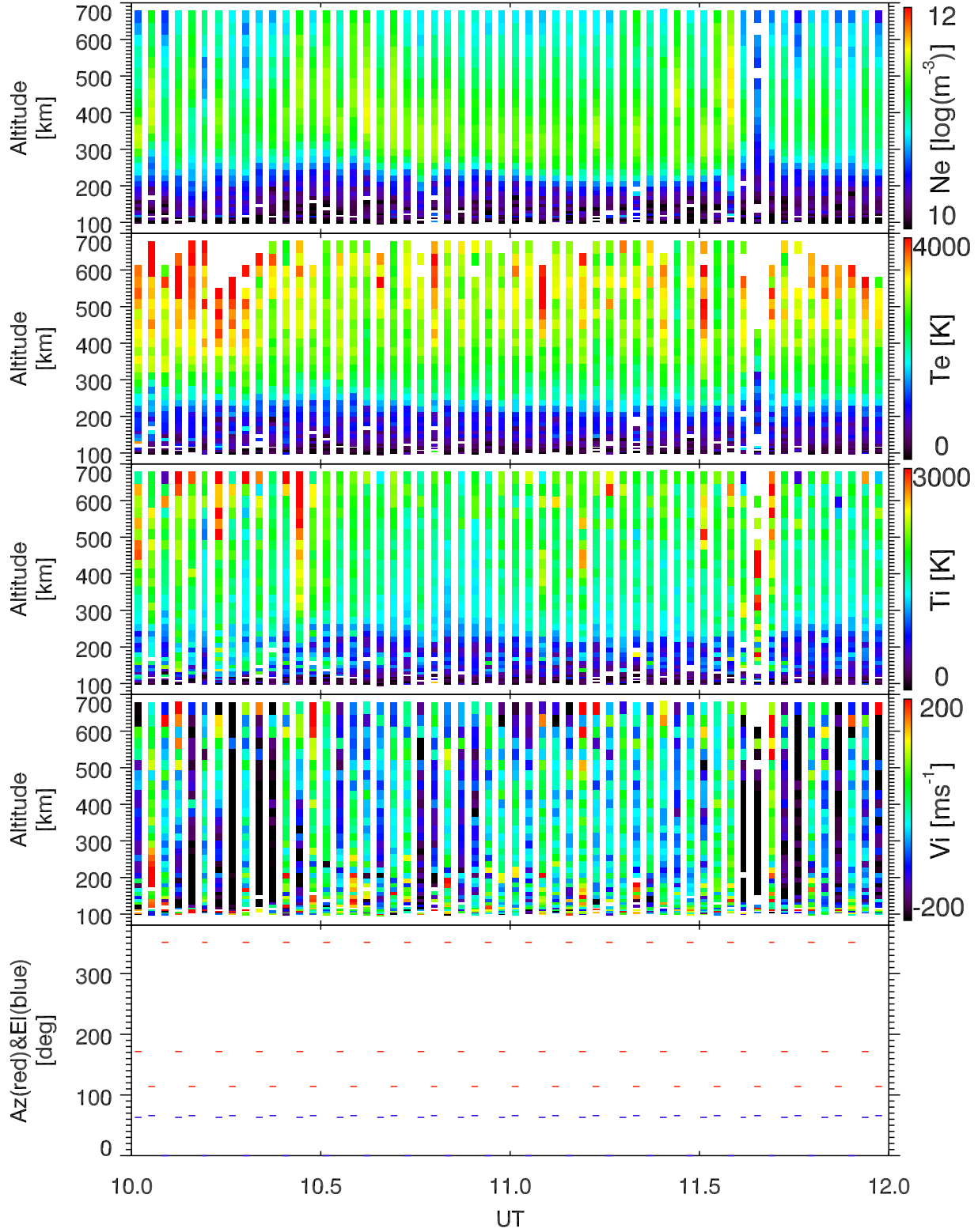
EISCAT 2002-11-02_10_12UT_tau0_ant@32m.
