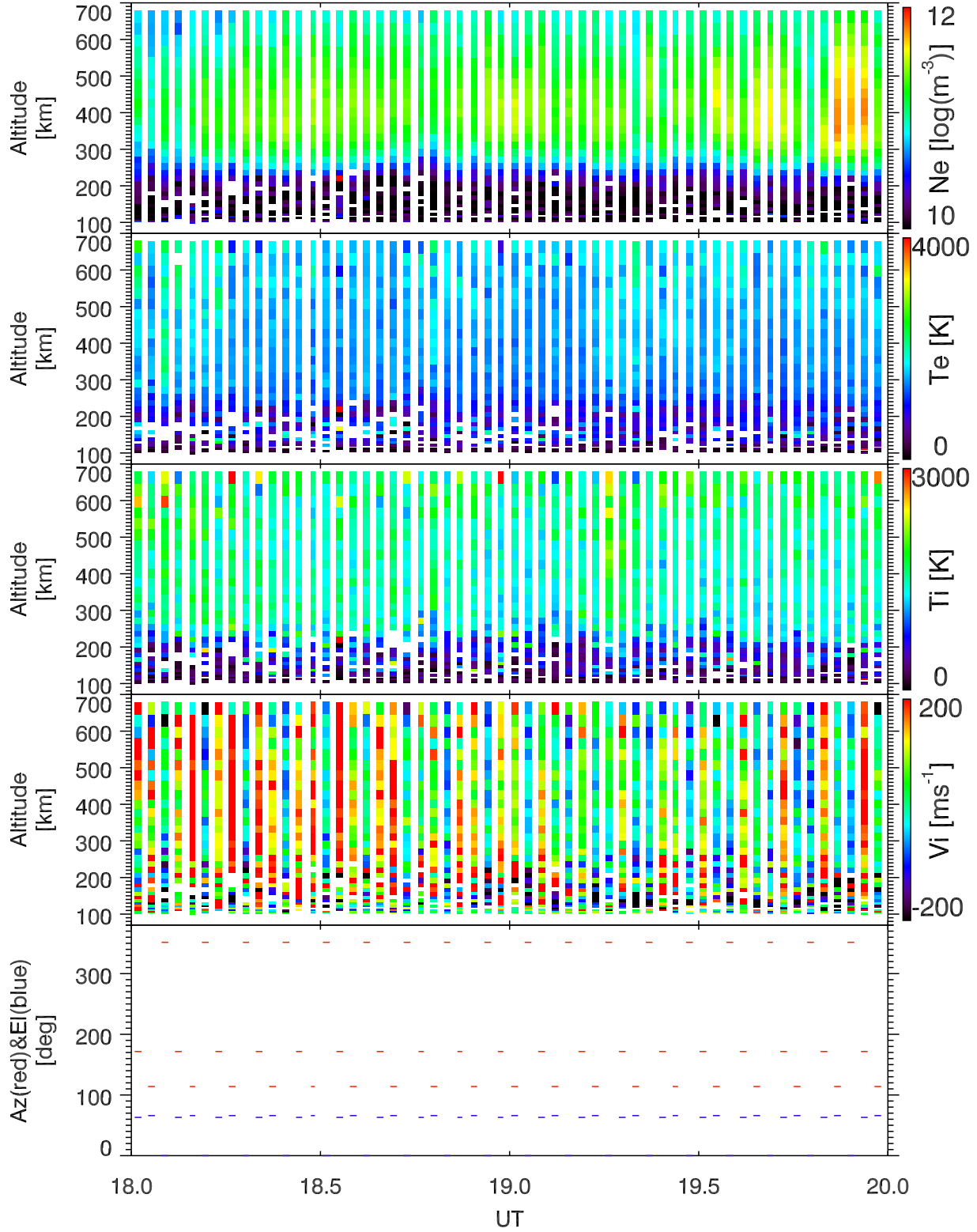
EISCAT 2002-11-02_18_20UT_tau0_ant@32m.
