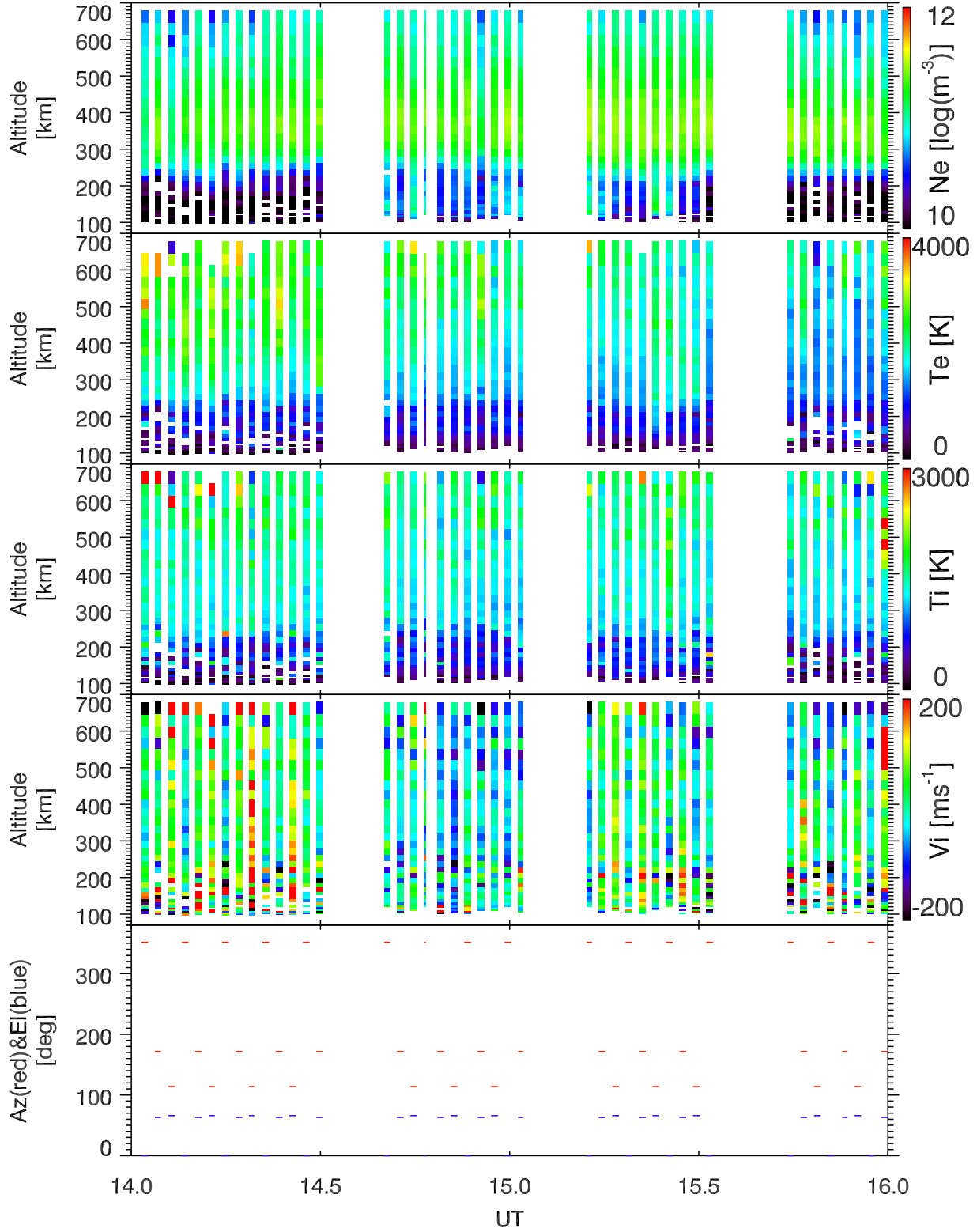
EISCAT 2002-11-03_14_16UT_tau0_all@32m.
