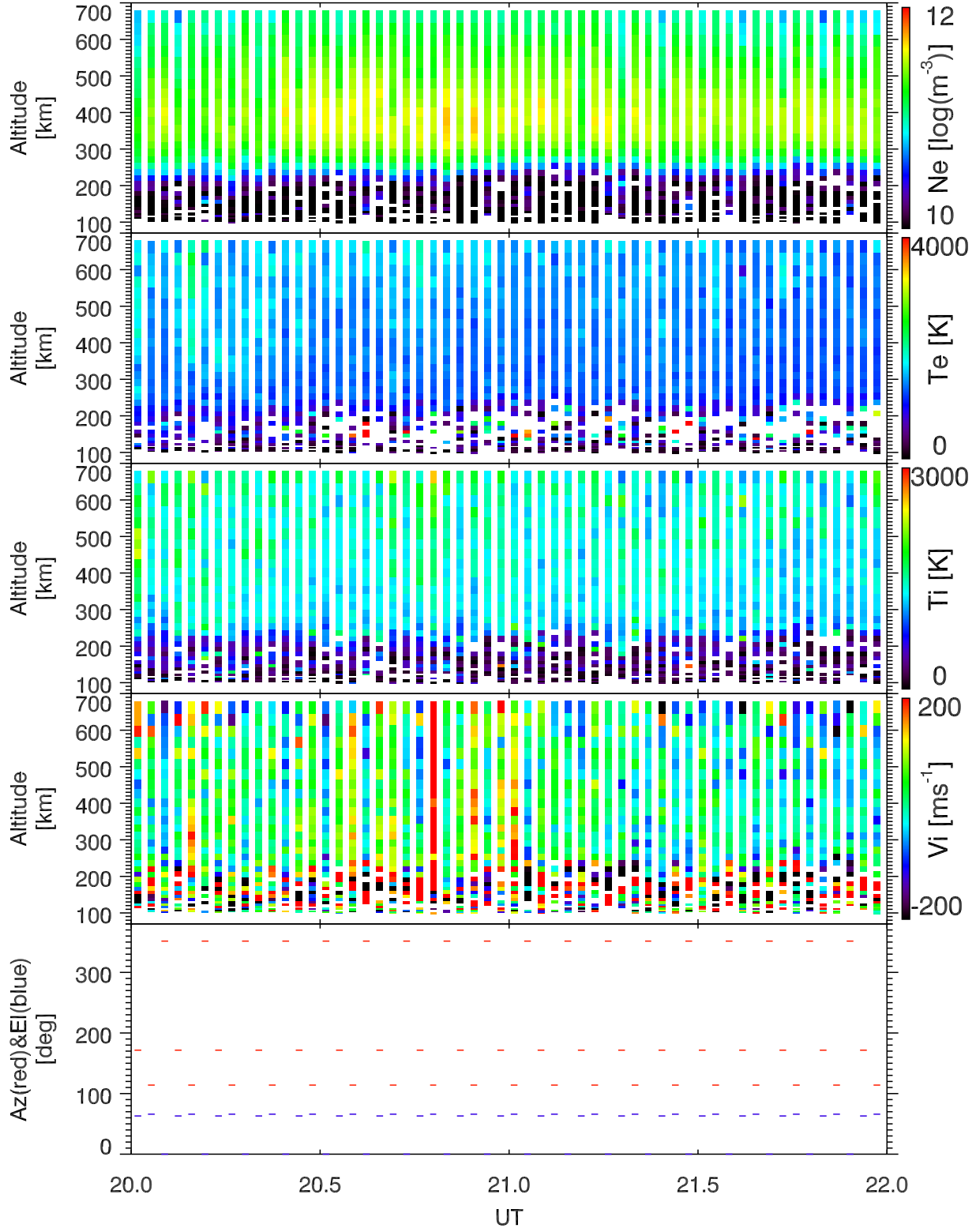
EISCAT 2002-11-11_20_22UT_tau0_ant@32m.
